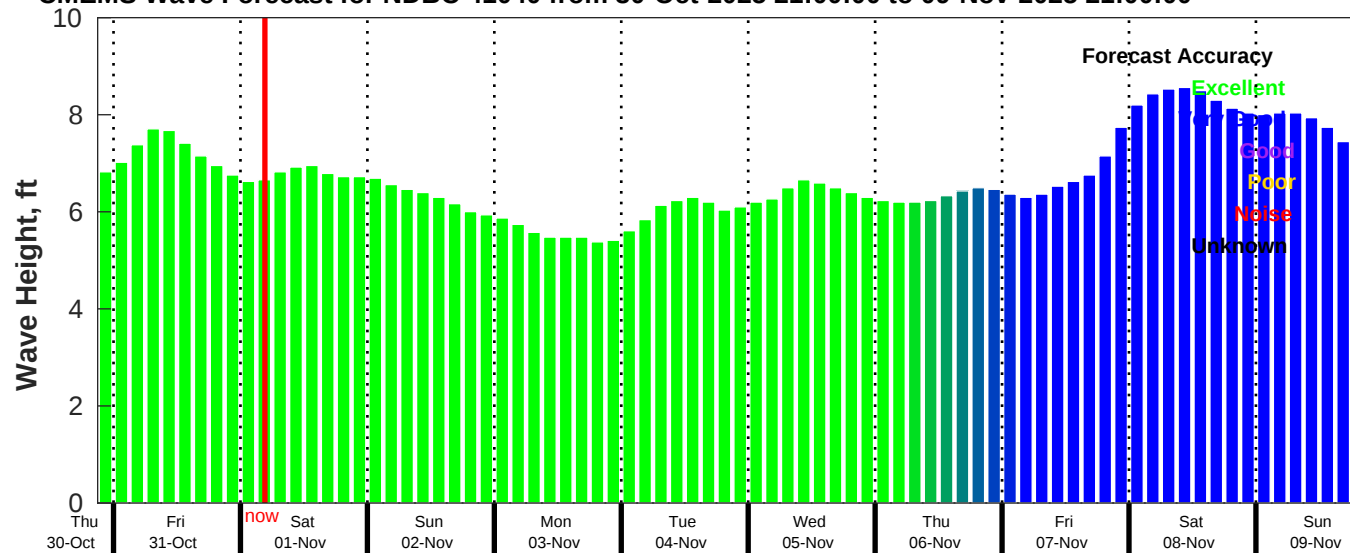
CMEMS Wave Forecast for NDBC 41040 from 30-Oct-2025 21:00:00 to 09-Nov-2025 21:00:00
