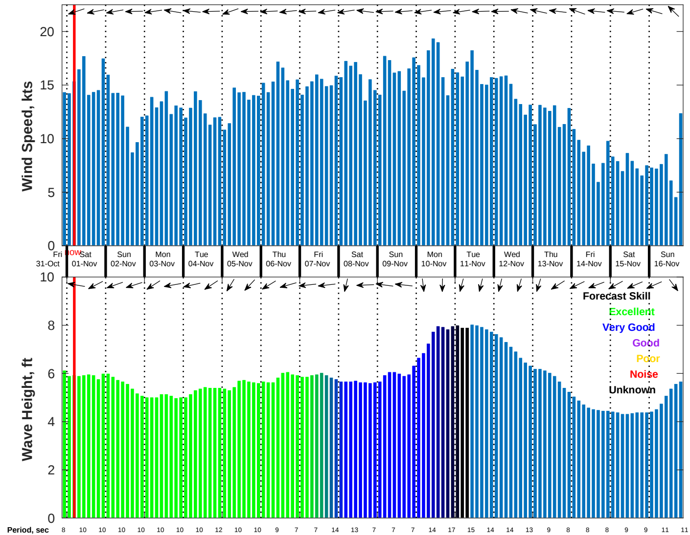
Wind & Wave Forecast for NDBC 41040 from 31-Oct-2025 21:00:00 to 16-Nov-2025 21:00:00
