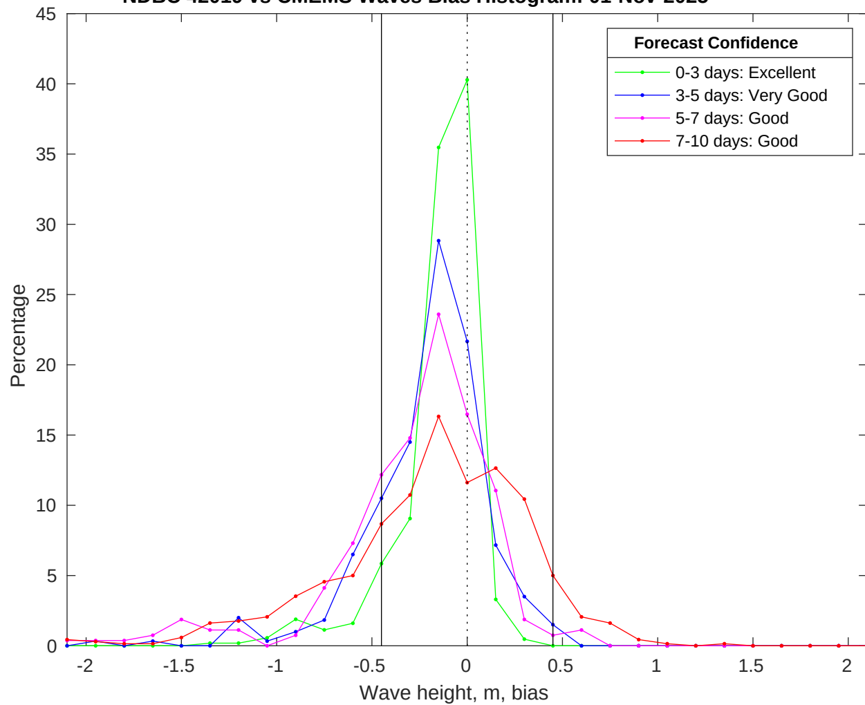
NDBC 42019 vs CMEMS Waves Bias Histogram: 01-Nov-2025
