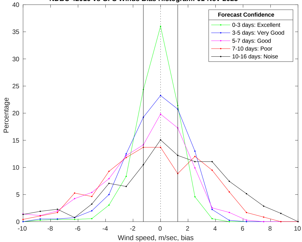
NDBC 42019 vs GFS Winds Bias Histogram: 01-Nov-2025
