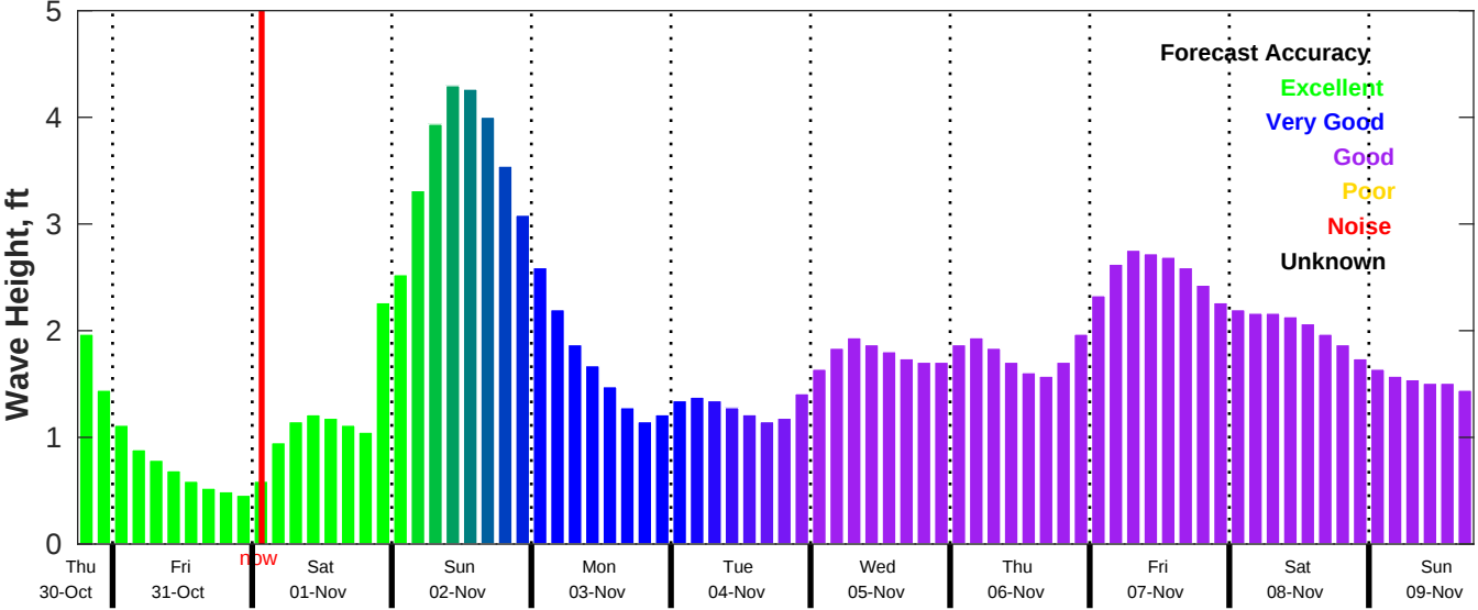
CMEMS Wave Forecast for NDBC 42019 from 30-Oct-2025 18:00:00 to 09-Nov-2025 18:00:00
