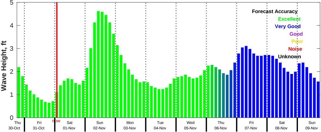
CMEMS Wave Forecast for NDBC 42020 from 30-Oct-2025 18:00:00 to 09-Nov-2025 18:00:00
