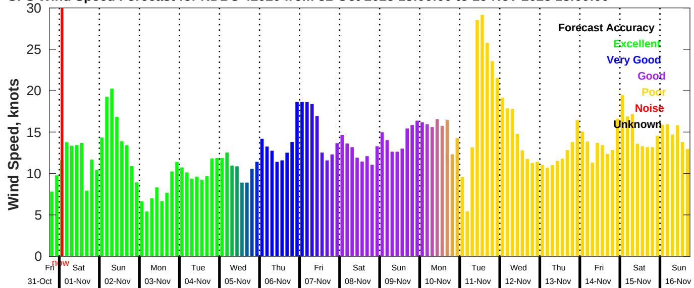
GFS Wind Speed Forecast for NDBC 42020 from 31-Oct-2025 18:00:00 to 16-Nov-2025 18:00:00
