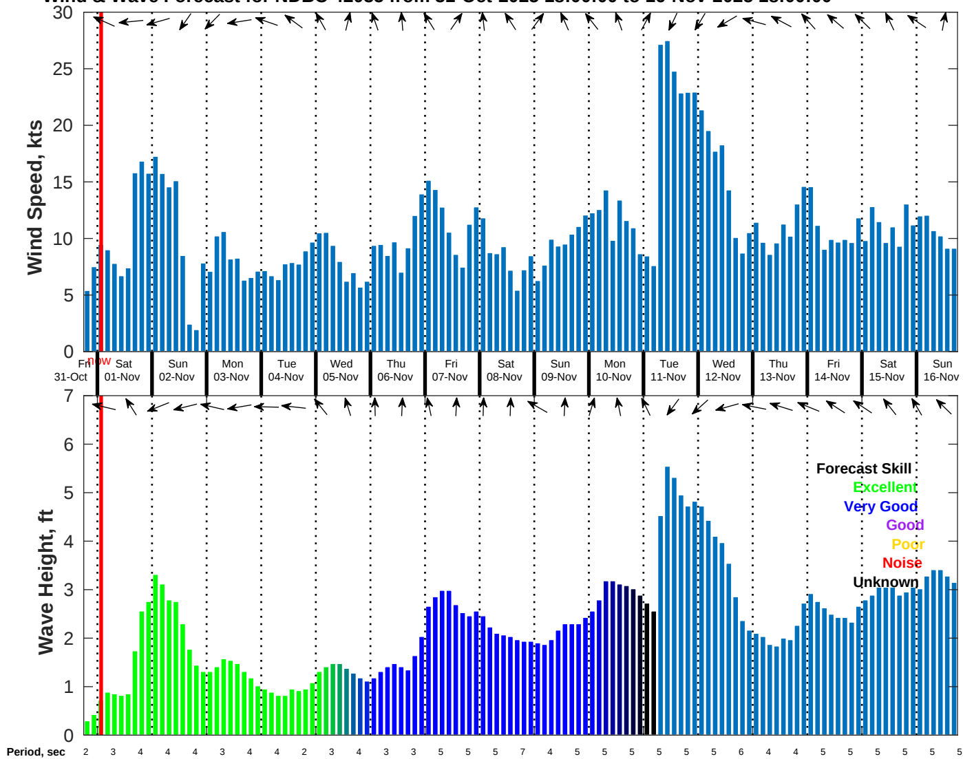
Wind & Wave Forecast for NDBC 42035 from 31-Oct-2025 18:00:00 to 16-Nov-2025 18:00:00
