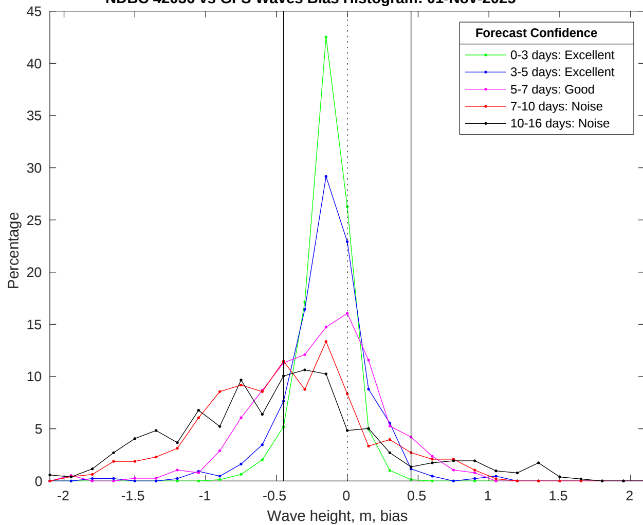
NDBC 42036 vs GFS Waves Bias Histogram: 01-Nov-2025
