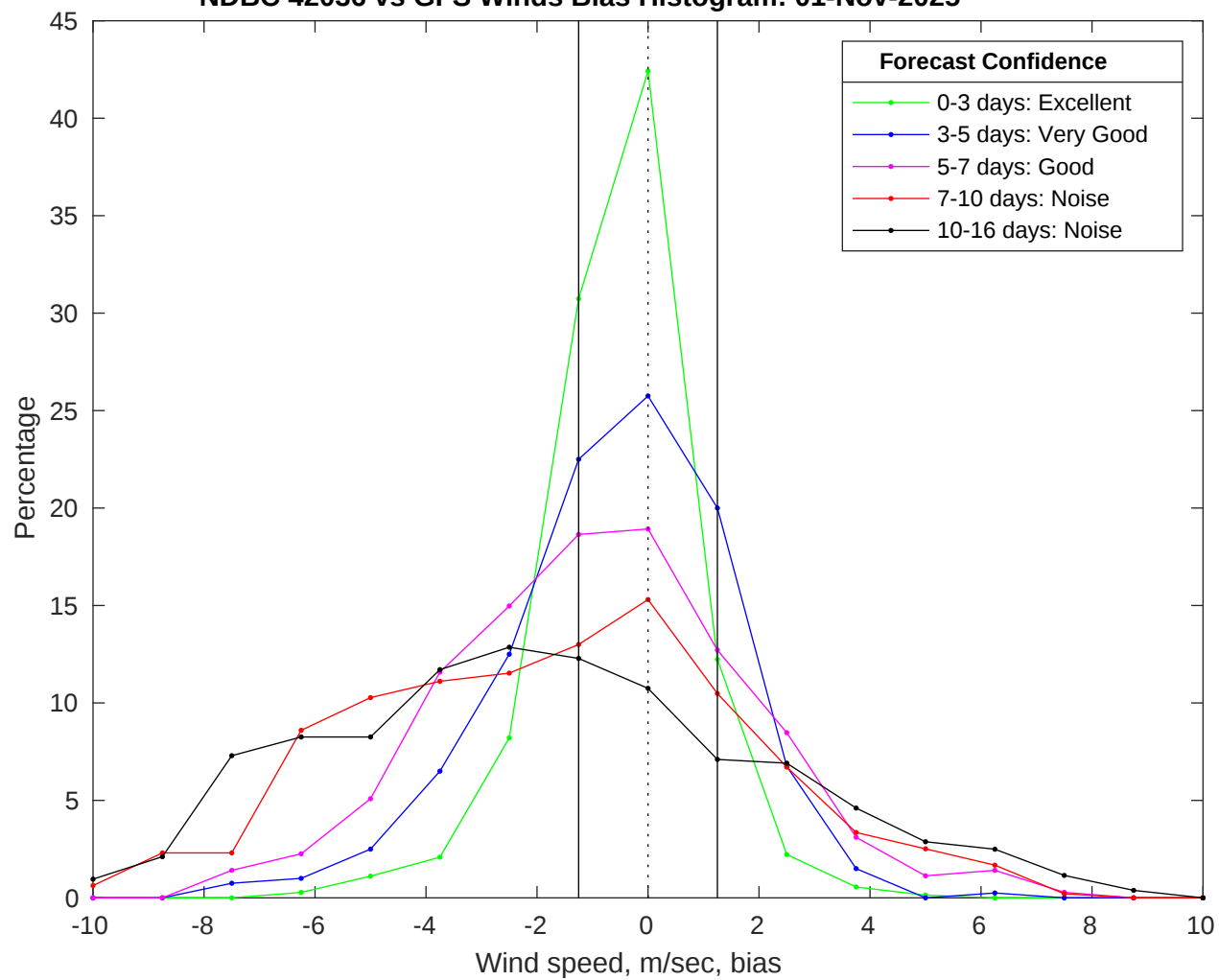
NDBC 42036 vs GFS Winds Bias Histogram: 01-Nov-2025
