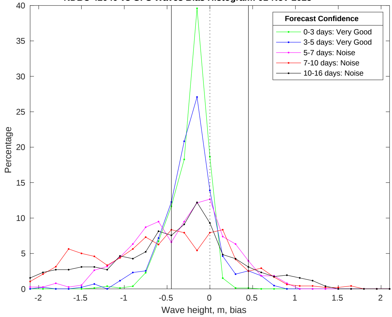
NDBC 42040 vs GFS Waves Bias Histogram: 01-Nov-2025
