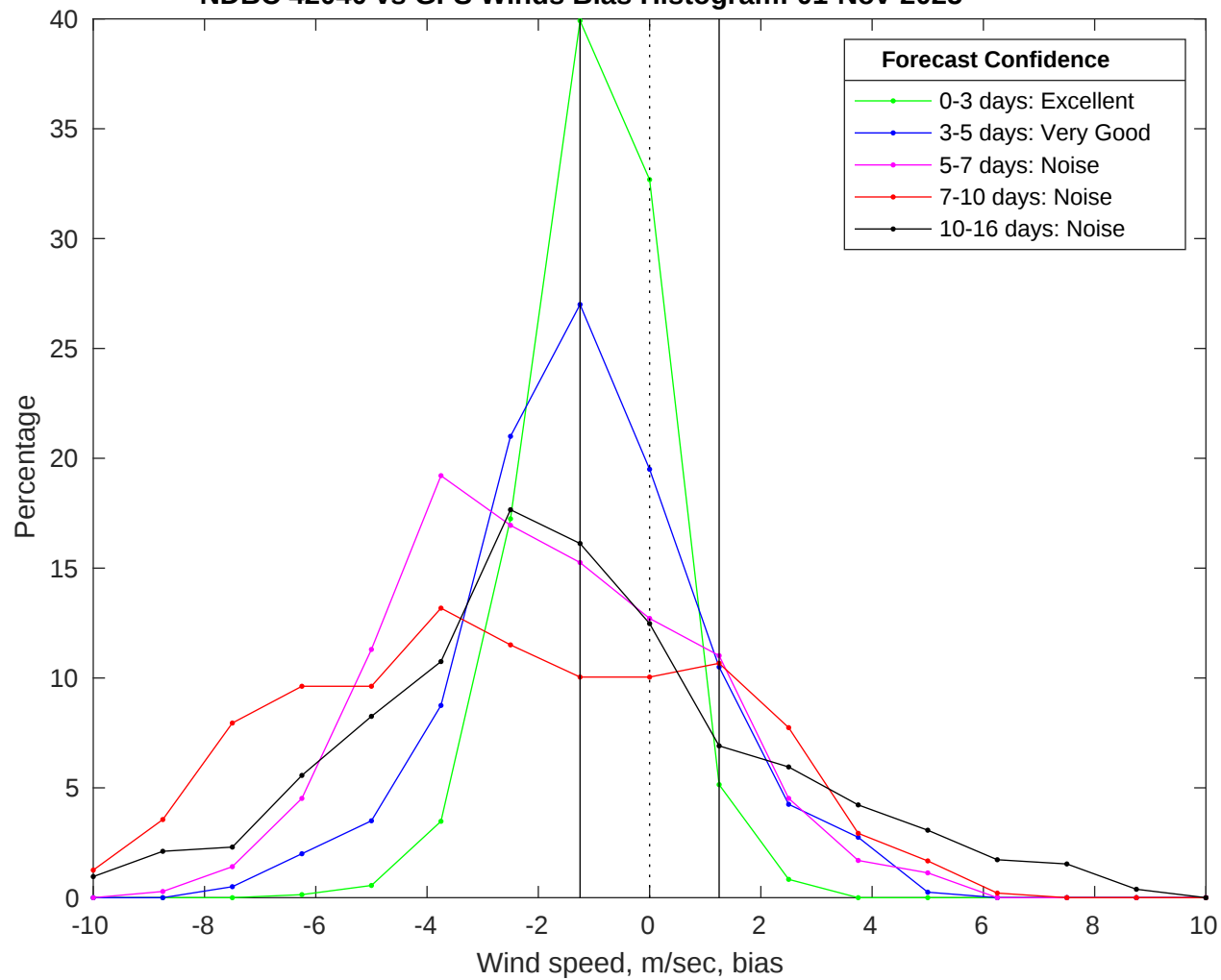
NDBC 42040 vs GFS Winds Bias Histogram: 01-Nov-2025
