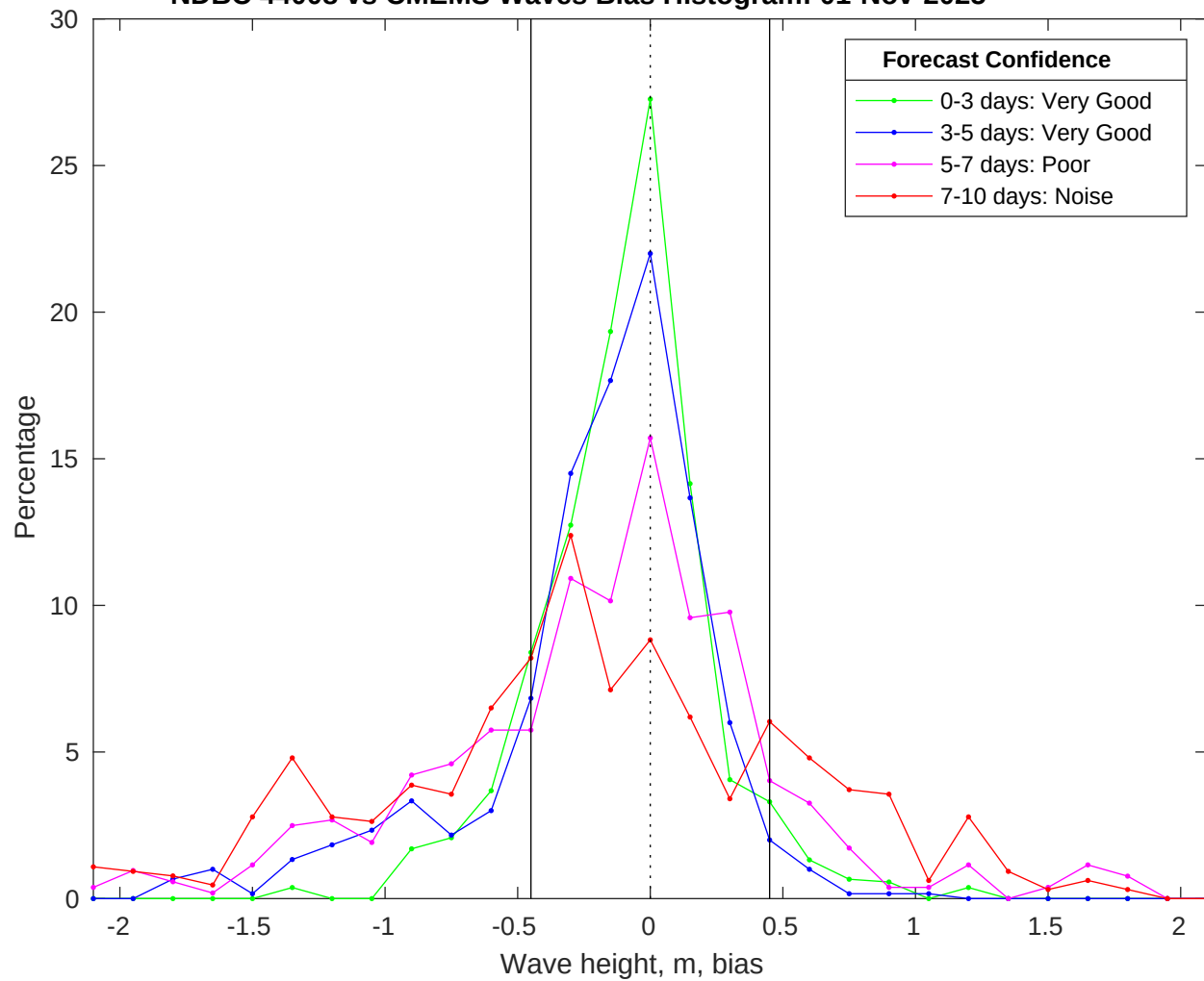
NDBC 44008 vs CMEMS Waves Bias Histogram: 01-Nov-2025
