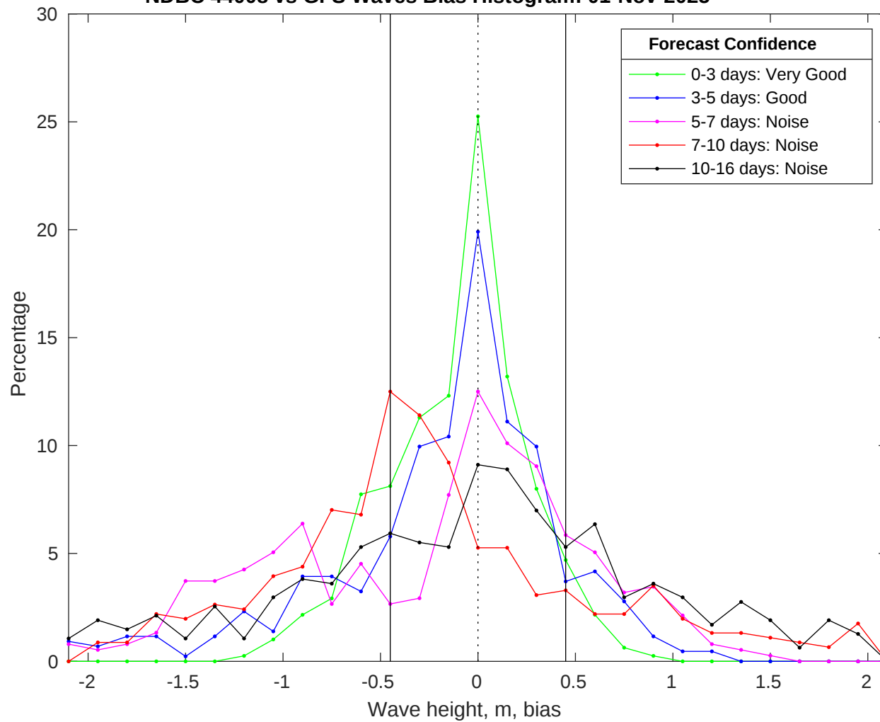
NDBC 44008 vs GFS Waves Bias Histogram: 01-Nov-2025
