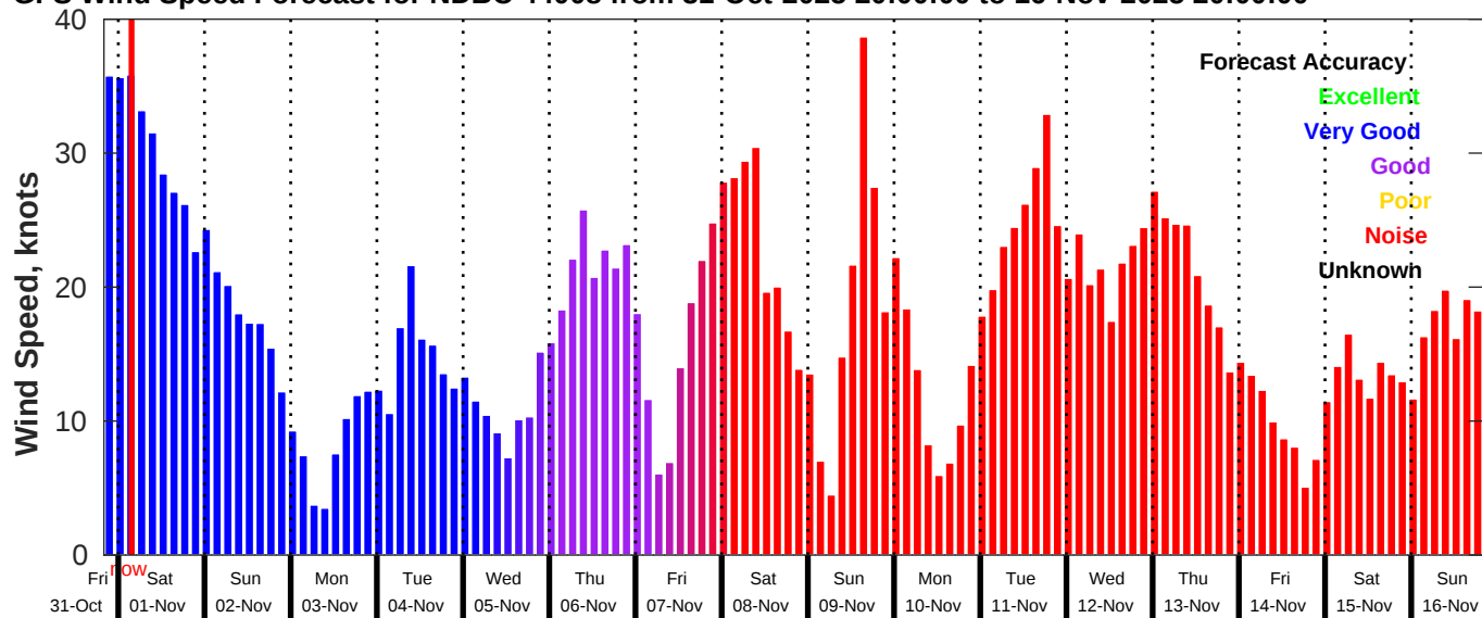
GFS Wind Speed Forecast for NDBC 44008 from 31-Oct-2025 20:00:00 to 16-Nov-2025 20:00:00
