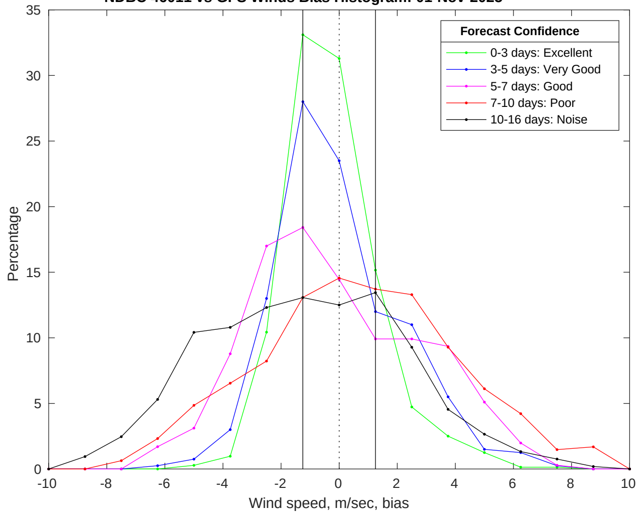
NDBC 46011 vs GFS Winds Bias Histogram: 01-Nov-2025
