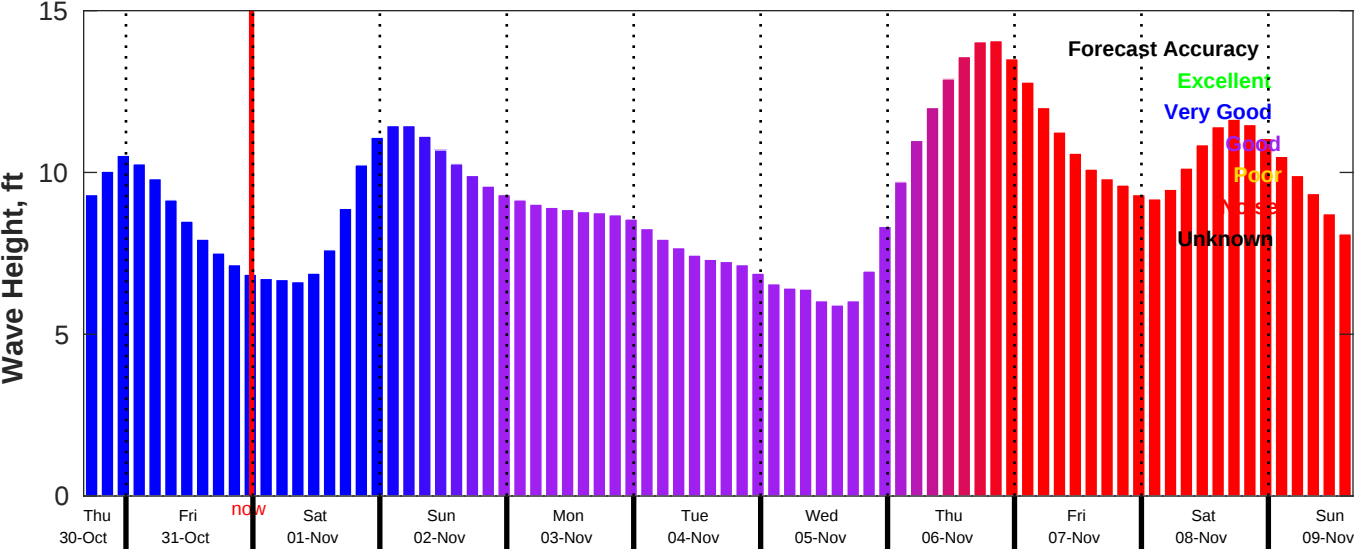
CMEMS Wave Forecast for NDBC 46011 from 30-Oct-2025 16:00:00 to 09-Nov-2025 16:00:00
