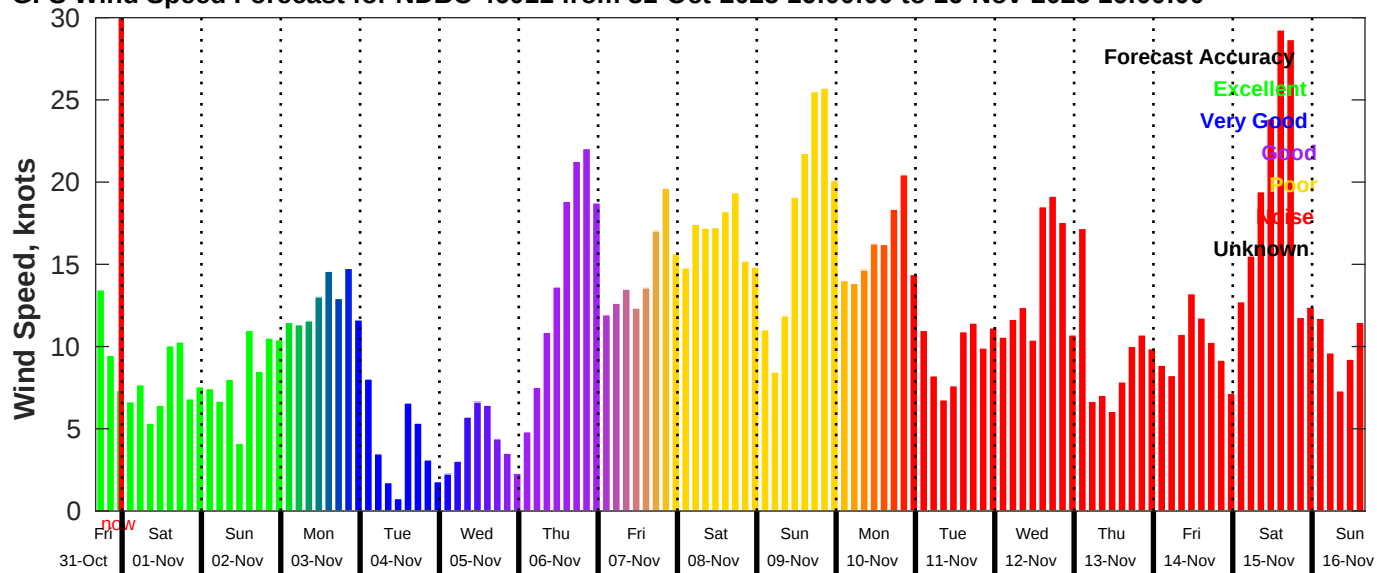
GFS Wind Speed Forecast for NDBC 46011 from 31-Oct-2025 16:00:00 to 16-Nov-2025 16:00:00
