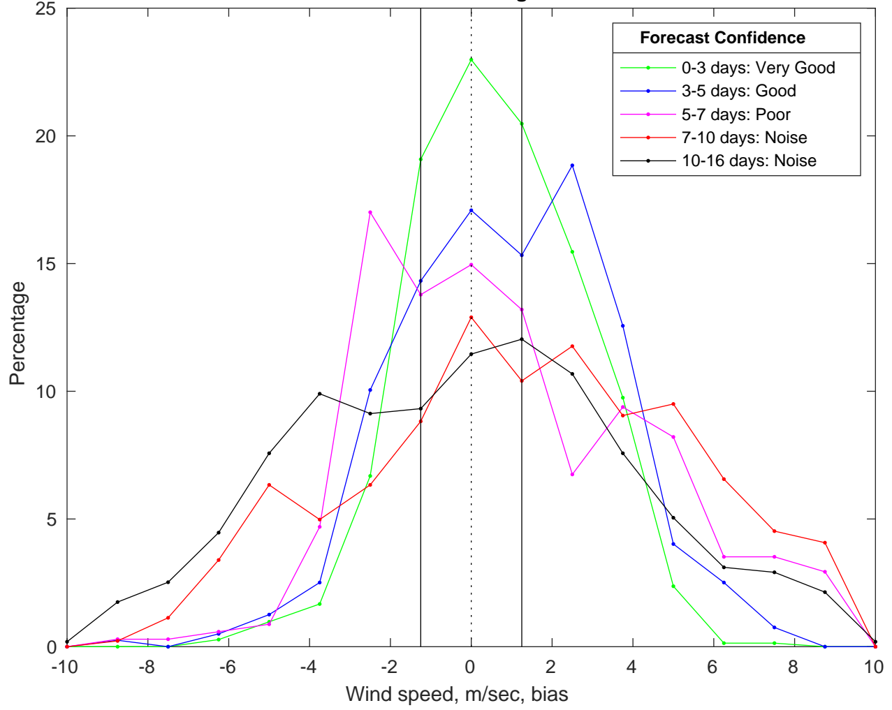
NDBC 46028 vs GFS Winds Bias Histogram: 01-Nov-2025
