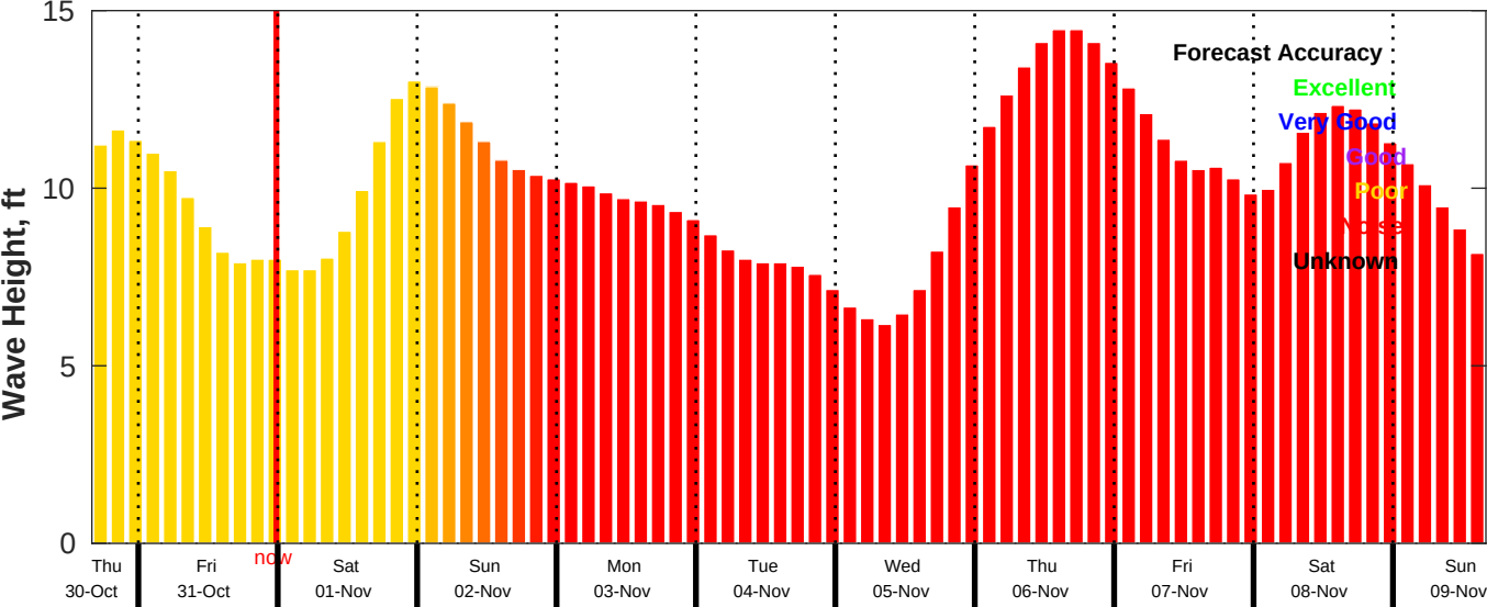
CMEMS Wave Forecast for NDBC 46028 from 30-Oct-2025 16:00:00 to 09-Nov-2025 16:00:00
