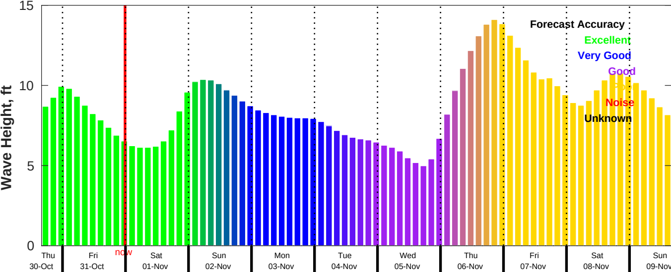
CMEMS Wave Forecast for NDBC 46054 from 30-Oct-2025 16:00:00 to 09-Nov-2025 16:00:00
