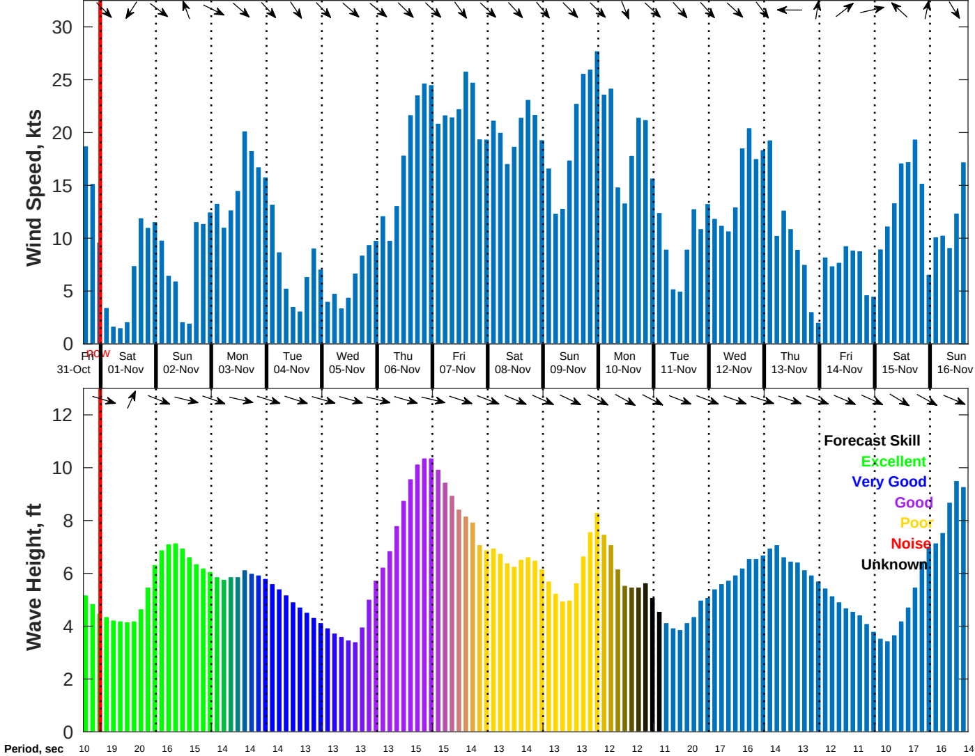
Wind & Wave Forecast for NDBC 46054 from 31-Oct-2025 16:00:00 to 16-Nov-2025 16:00:00
