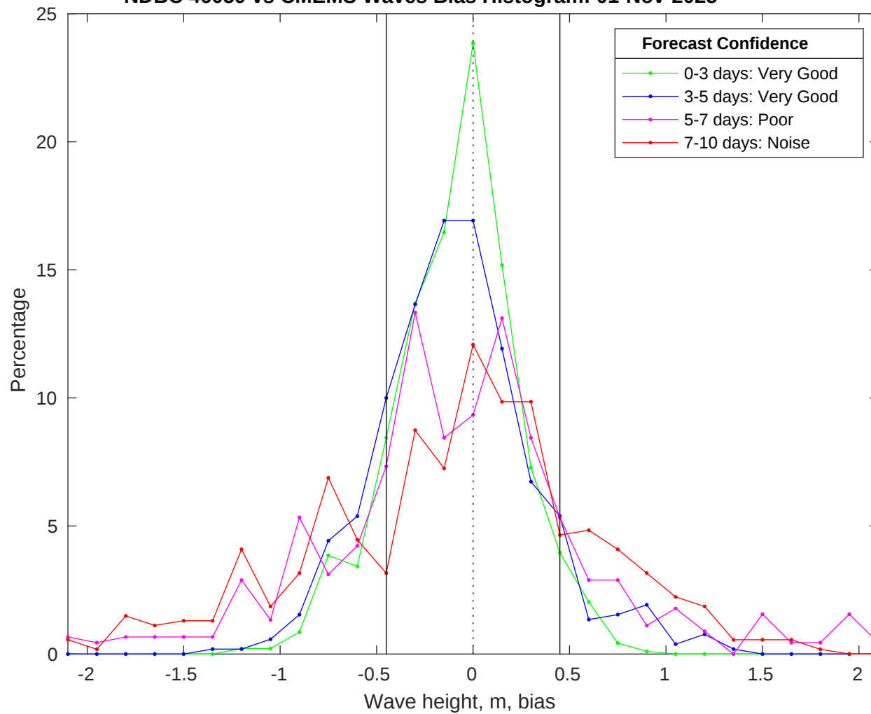
NDBC 46059 vs CMEMS Waves Bias Histogram: 01-Nov-2025
