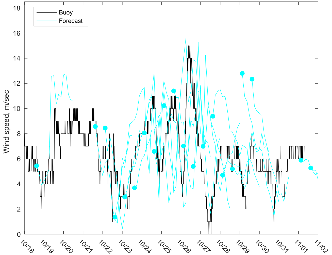
NDBC 46059 vs GFS Winds: 5 to 7 day forecast
