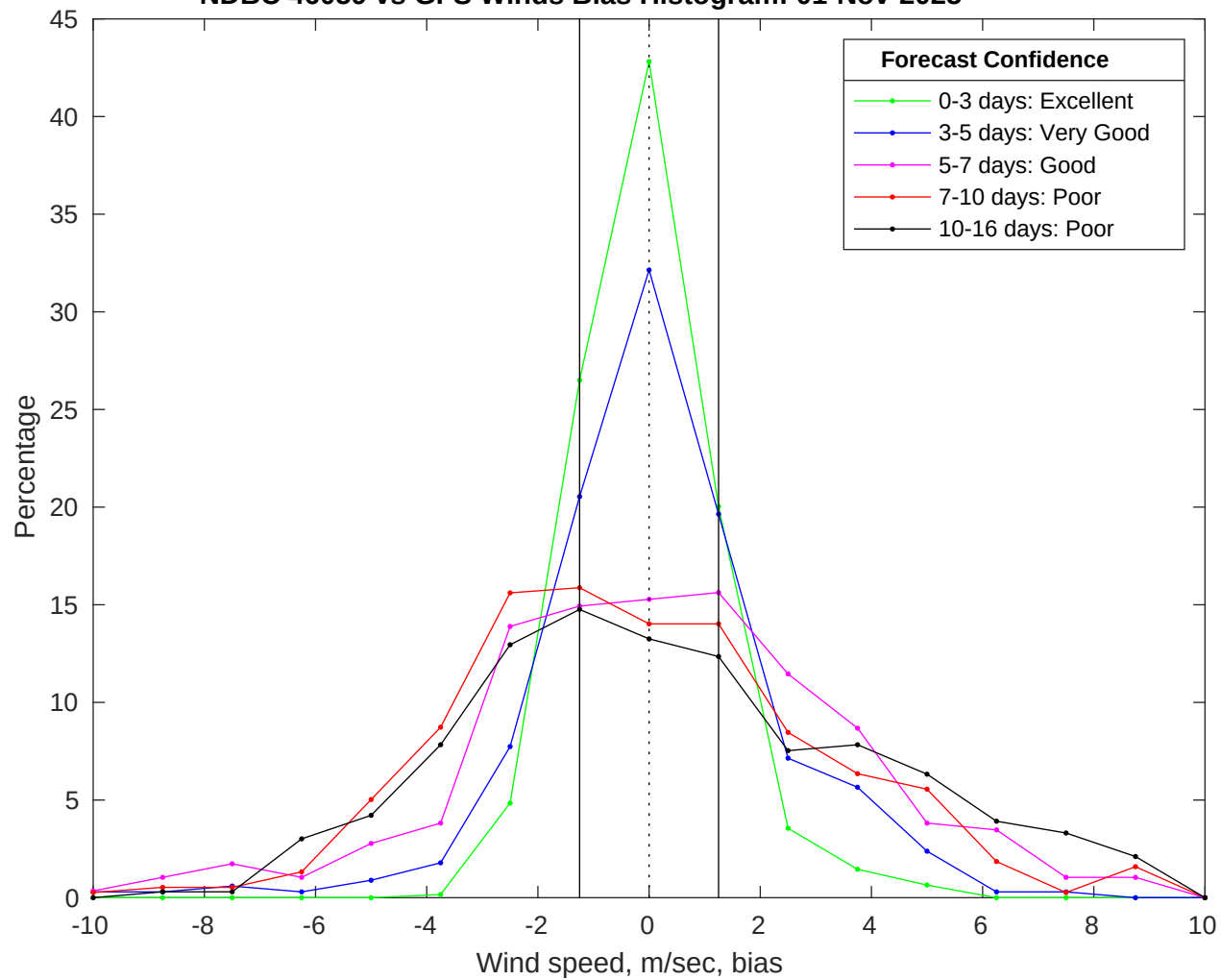
NDBC 46059 vs GFS Winds Bias Histogram: 01-Nov-2025
