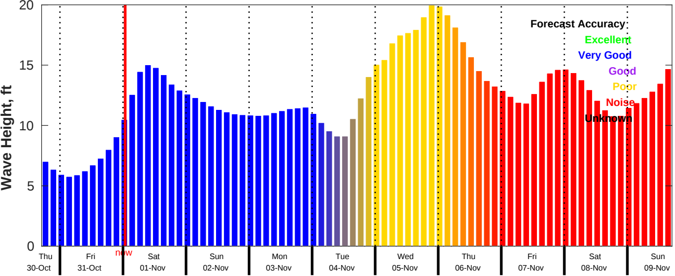
CMEMS Wave Forecast for NDBC 46059 from 30-Oct-2025 17:00:00 to 09-Nov-2025 17:00:00
