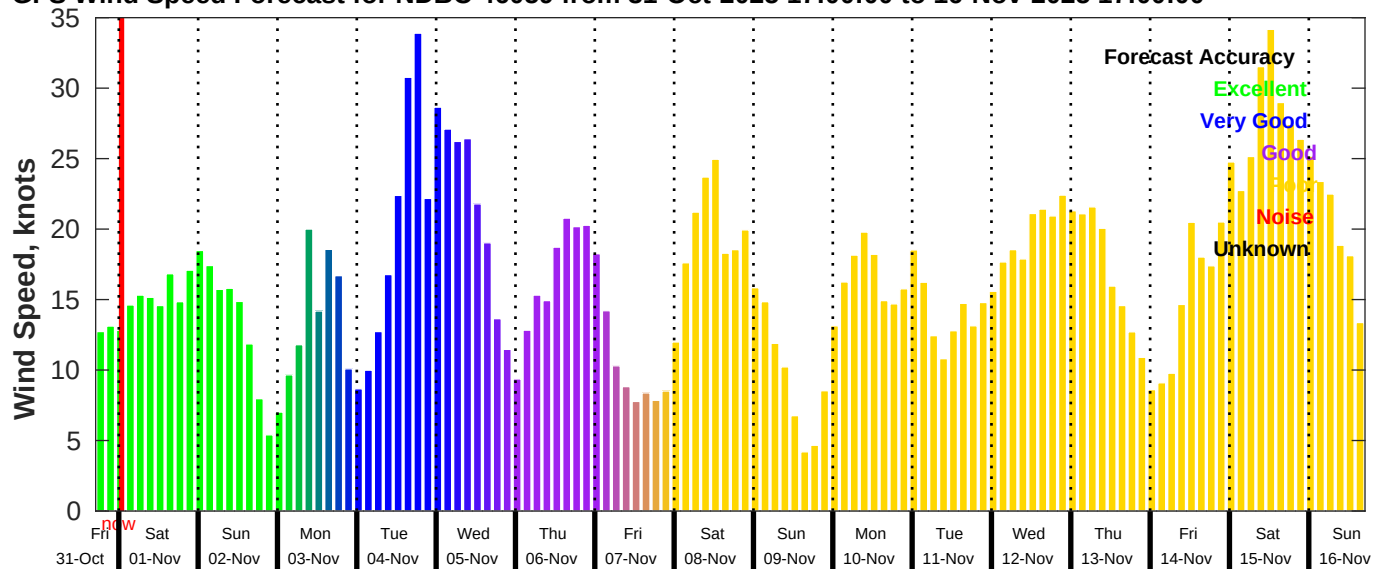
GFS Wind Speed Forecast for NDBC 46059 from 31-Oct-2025 17:00:00 to 16-Nov-2025 17:00:00
