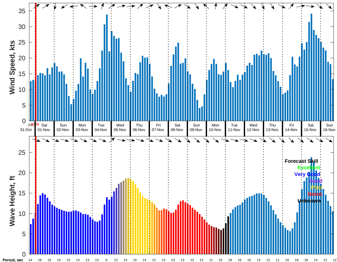
Wind & Wave Forecast for NDBC 46059 from 31-Oct-2025 17:00:00 to 16-Nov-2025 17:00:00
