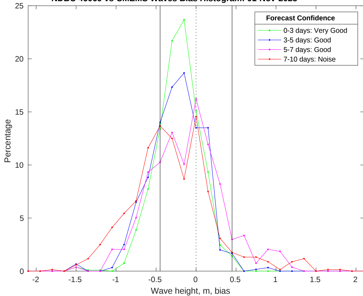
NDBC 46069 vs CMEMS Waves Bias Histogram: 01-Nov-2025
