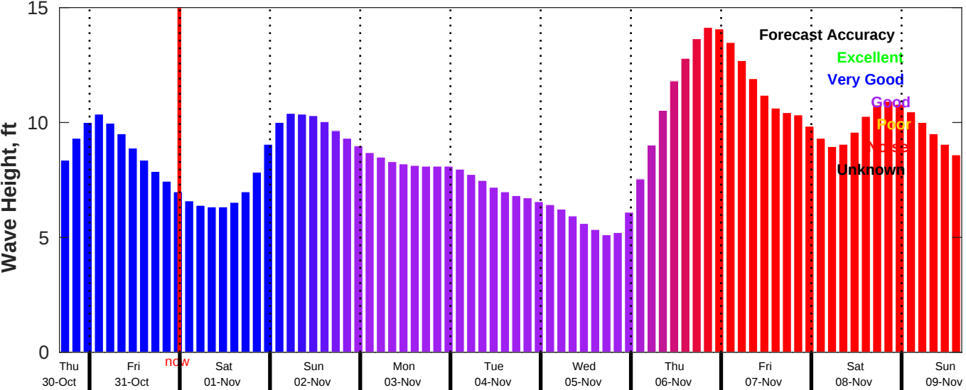
CMEMS Wave Forecast for NDBC 46069 from 30-Oct-2025 16:00:00 to 09-Nov-2025 16:00:00
