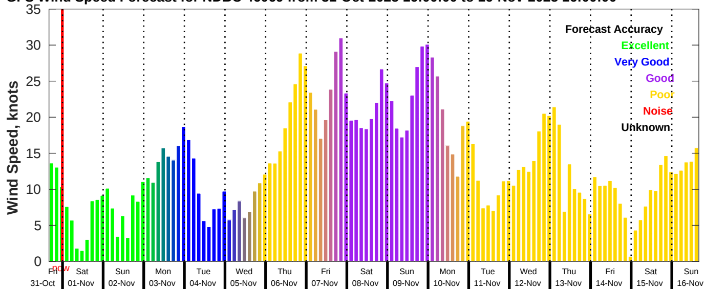
GFS Wind Speed Forecast for NDBC 46069 from 31-Oct-2025 16:00:00 to 16-Nov-2025 16:00:00
