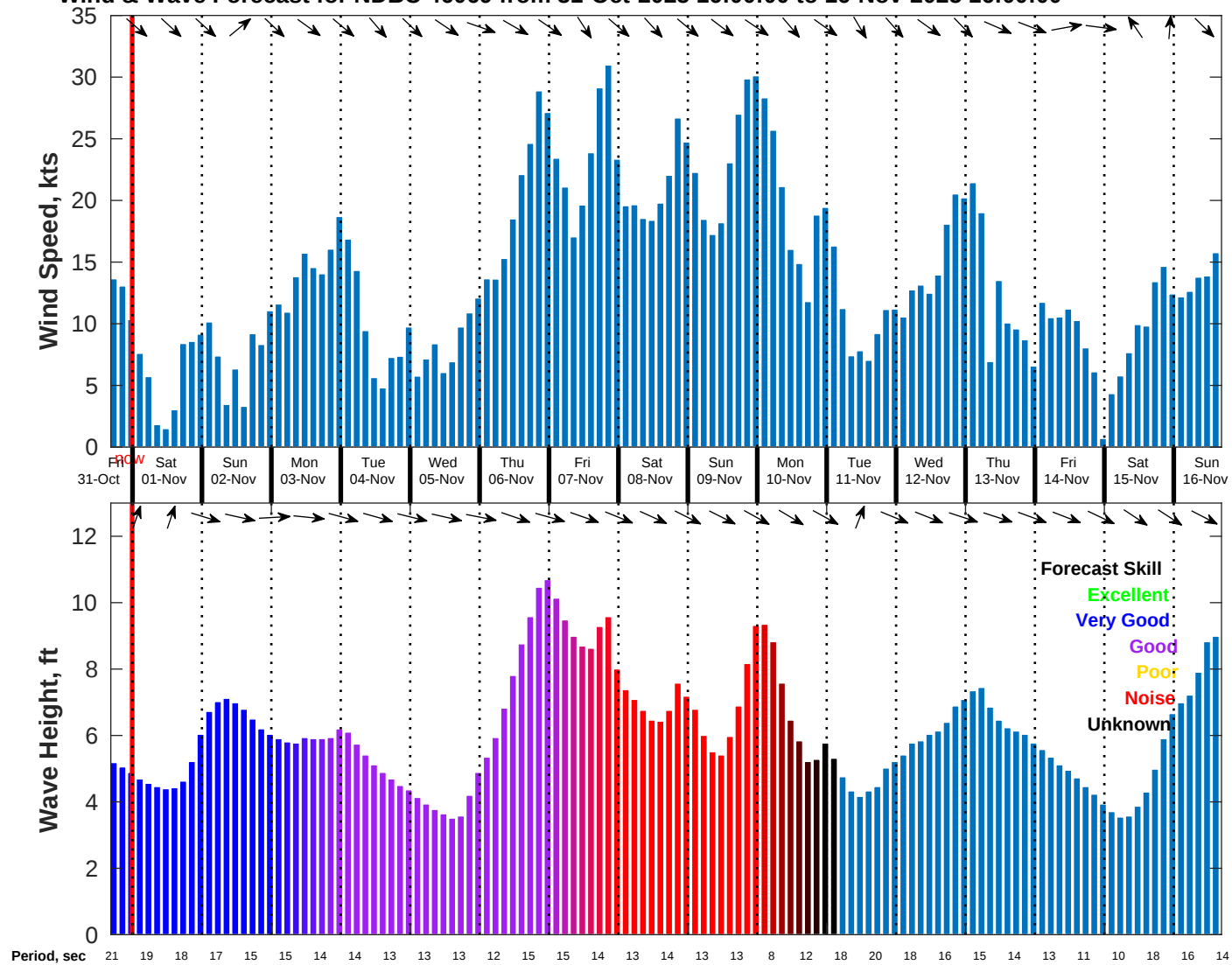
Wind & Wave Forecast for NDBC 46069 from 31-Oct-2025 16:00:00 to 16-Nov-2025 16:00:00
