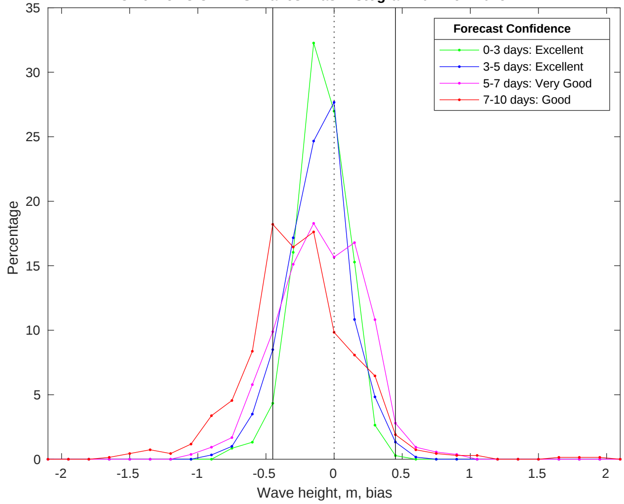
NDBC 46215 vs CMEMS Waves Bias Histogram: 01-Nov-2025
