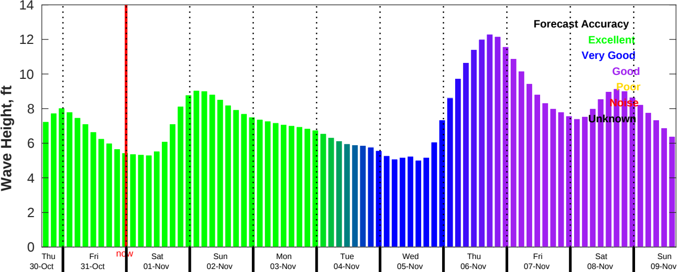
CMEMS Wave Forecast for NDBC 46215 from 30-Oct-2025 16:00:00 to 09-Nov-2025 16:00:00
