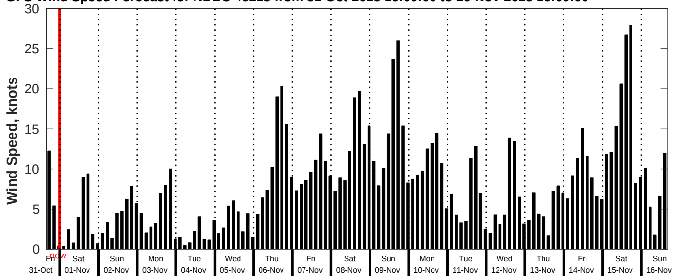
GFS Wind Speed Forecast for NDBC 46215 from 31-Oct-2025 16:00:00 to 16-Nov-2025 16:00:00
