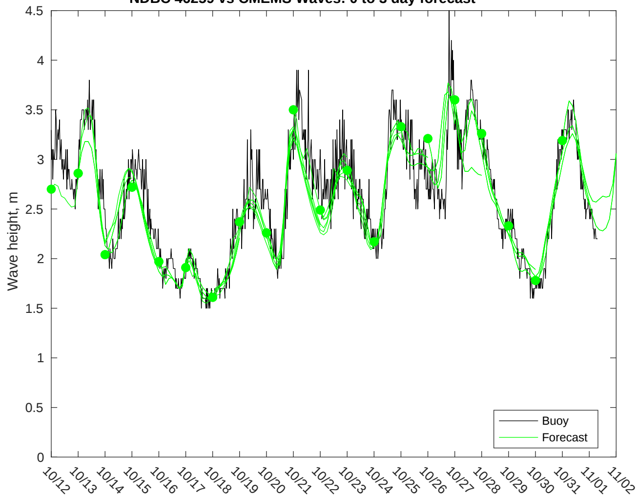
NDBC 46259 vs CMEMS Waves: 0 to 3 day forecast
