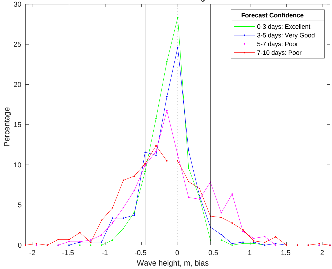
NDBC 46259 vs CMEMS Waves Bias Histogram: 01-Nov-2025
