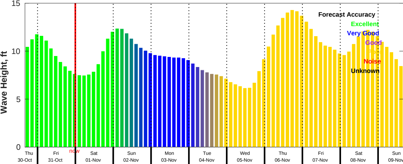
CMEMS Wave Forecast for NDBC 46259 from 30-Oct-2025 16:00:00 to 09-Nov-2025 16:00:00
