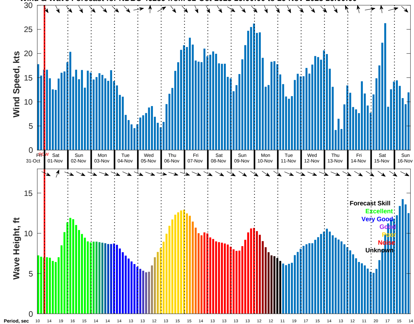
Wind & Wave Forecast for NDBC 46259 from 31-Oct-2025 16:00:00 to 16-Nov-2025 16:00:00
