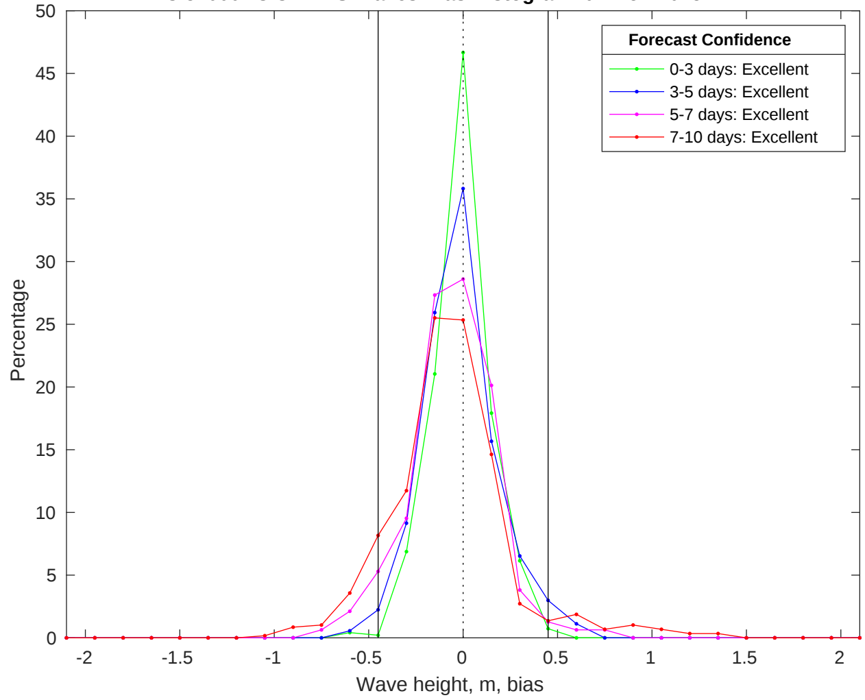
NDBC 51000 vs CMEMS Waves Bias Histogram: 01-Nov-2025
