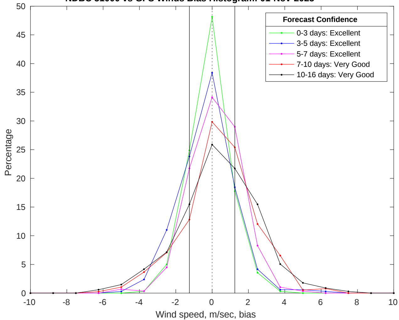
NDBC 51000 vs GFS Winds Bias Histogram: 01-Nov-2025
