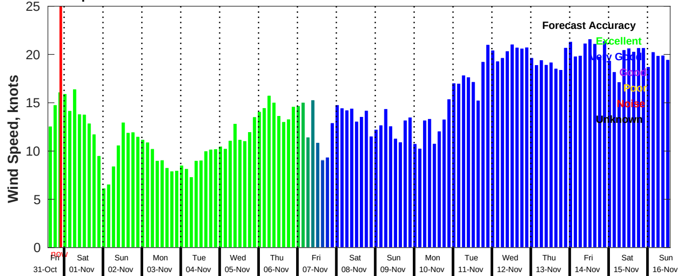
GFS Wind Speed Forecast for NDBC 51000 from 31-Oct-2025 14:00:00 to 16-Nov-2025 14:00:00
