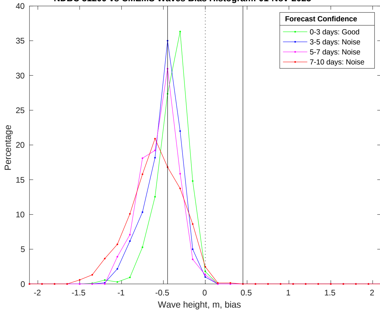
NDBC 51209 vs CMEMS Waves Bias Histogram: 01-Nov-2025
