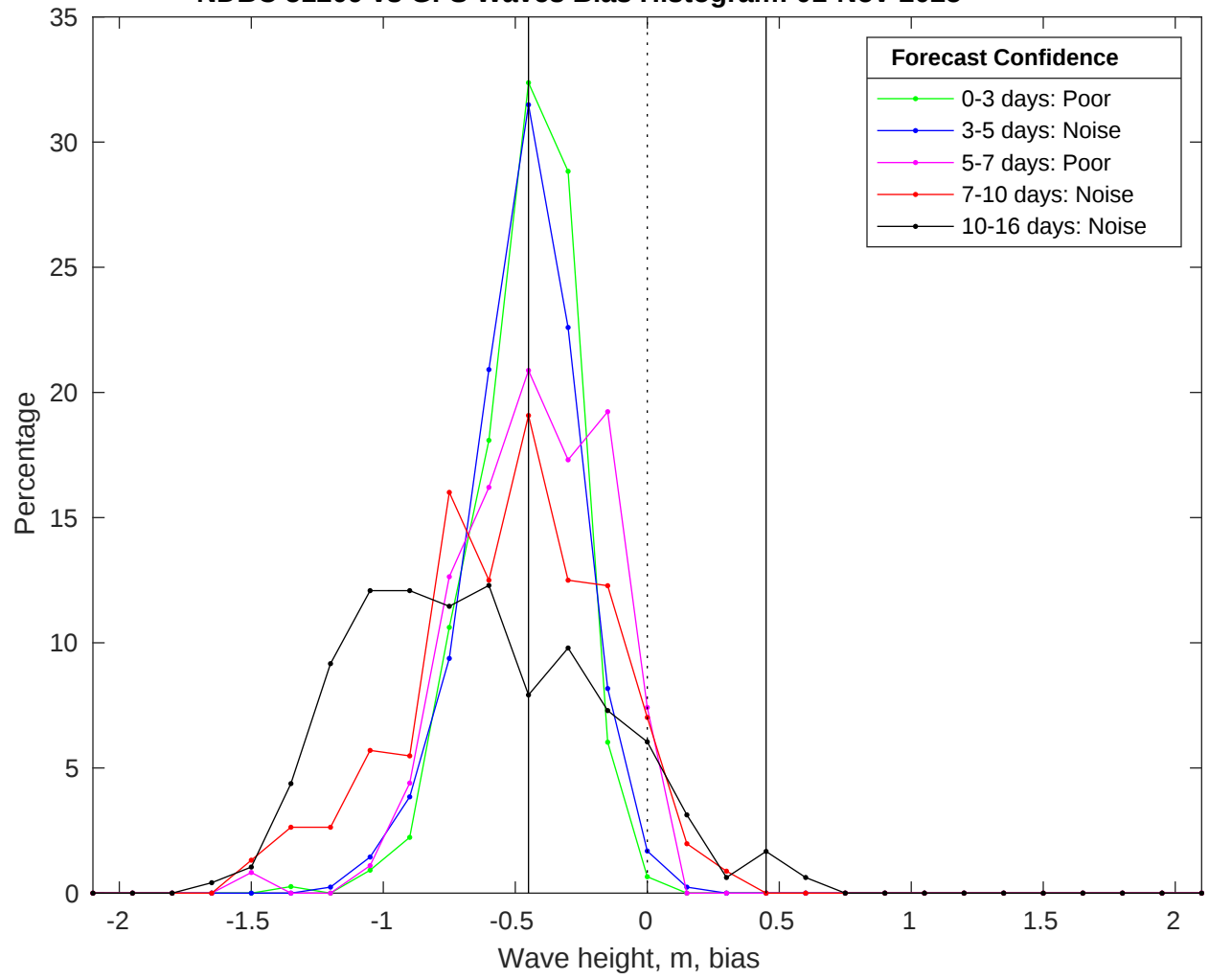
NDBC 51209 vs GFS Waves Bias Histogram: 01-Nov-2025
