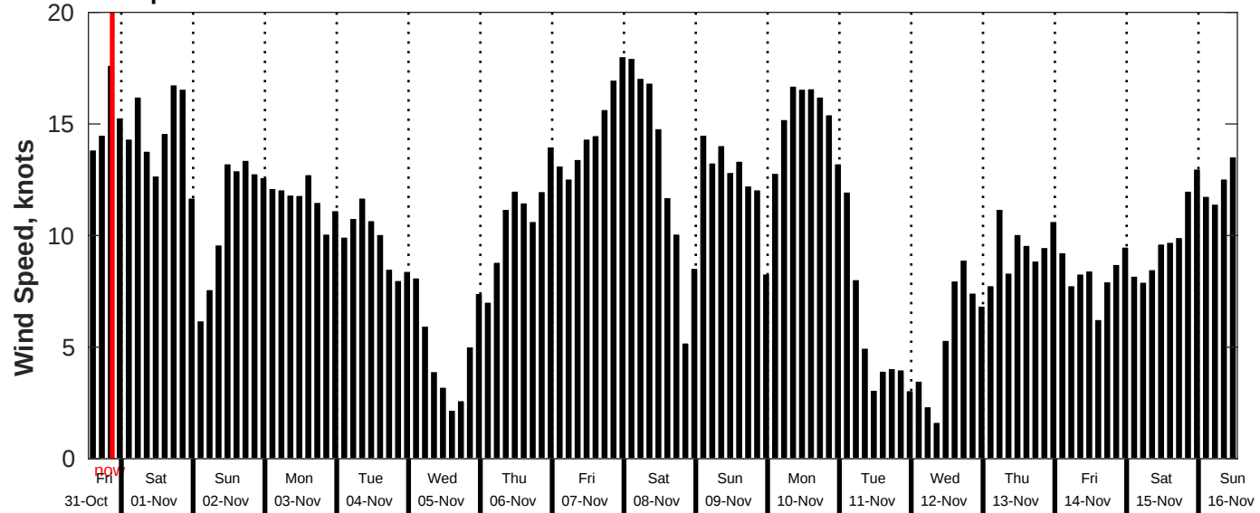
GFS Wind Speed Forecast for NDBC 51209 from 31-Oct-2025 13:00:00 to 16-Nov-2025 13:00:00
