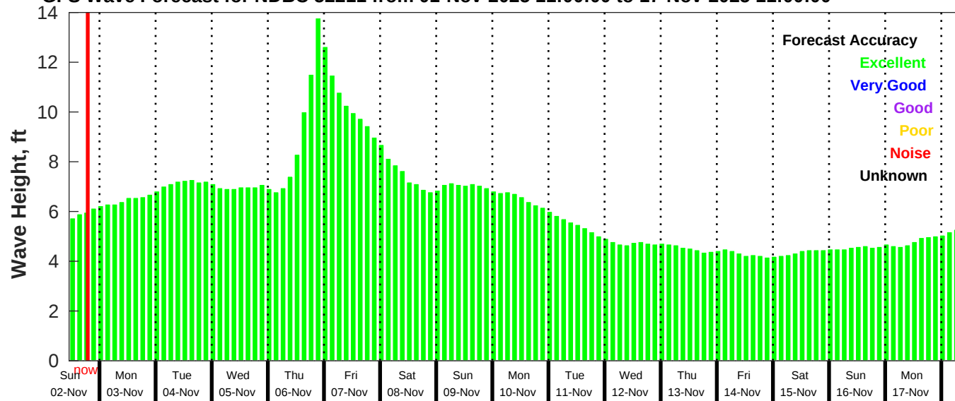
GFS Wave Forecast for NDBC 52211 from 01-Nov-2025 11:00:00 to 17-Nov-2025 11:00:00
