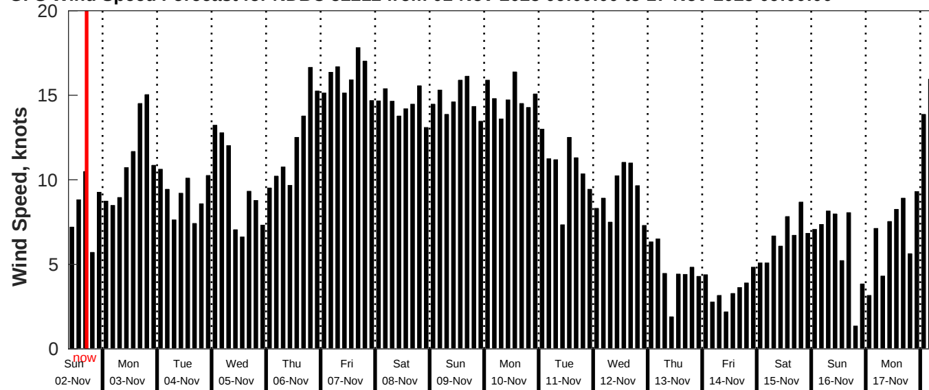
GFS Wind Speed Forecast for NDBC 52212 from 01-Nov-2025 09:00:00 to 17-Nov-2025 09:00:00
