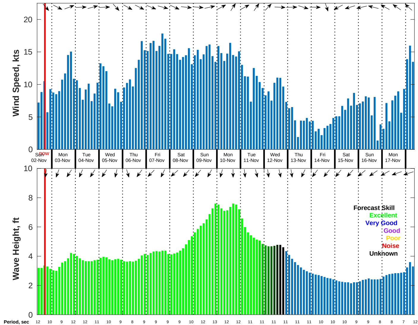
Wind & Wave Forecast for NDBC 52212 from 01-Nov-2025 09:00:00 to 17-Nov-2025 09:00:00
