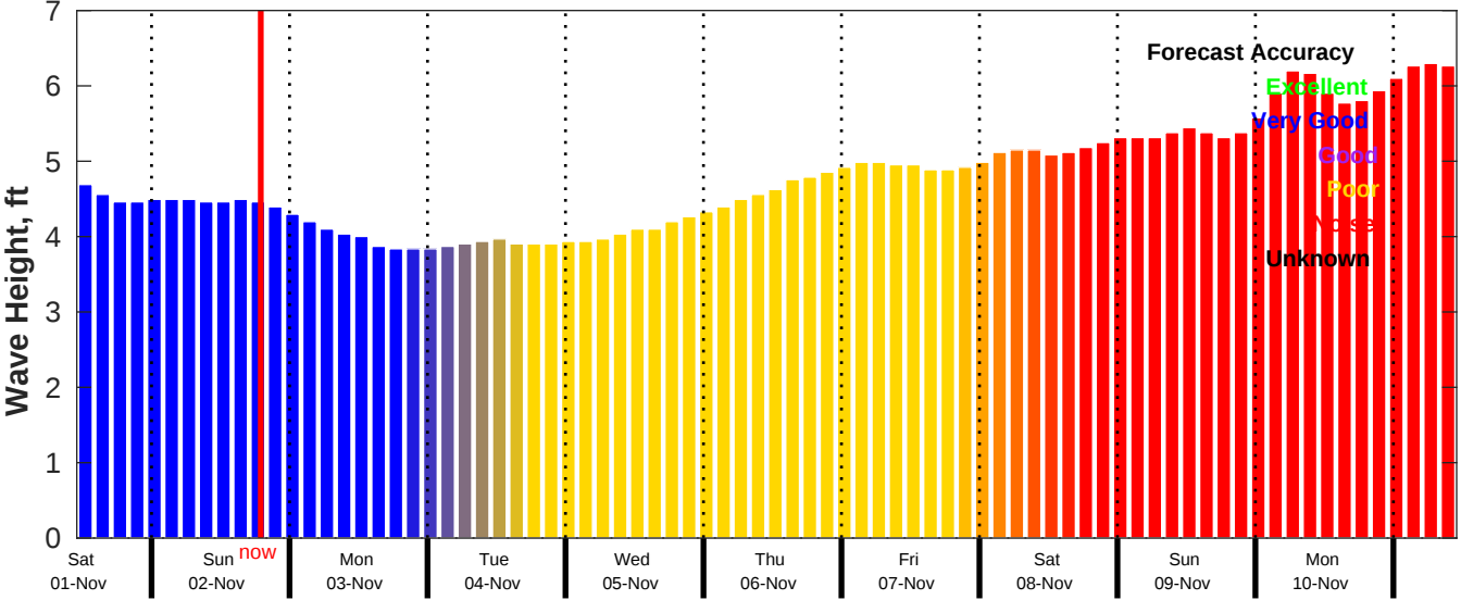
CMEMS Wave Forecast for NDBC 52213 from 31-Oct-2025 11:00:00 to 10-Nov-2025 11:00:00
