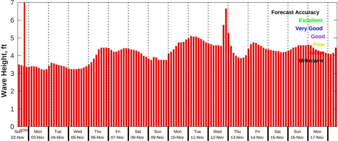
GFS Wave Forecast for NDBC 52213 from 01-Nov-2025 11:00:00 to 17-Nov-2025 11:00:00
